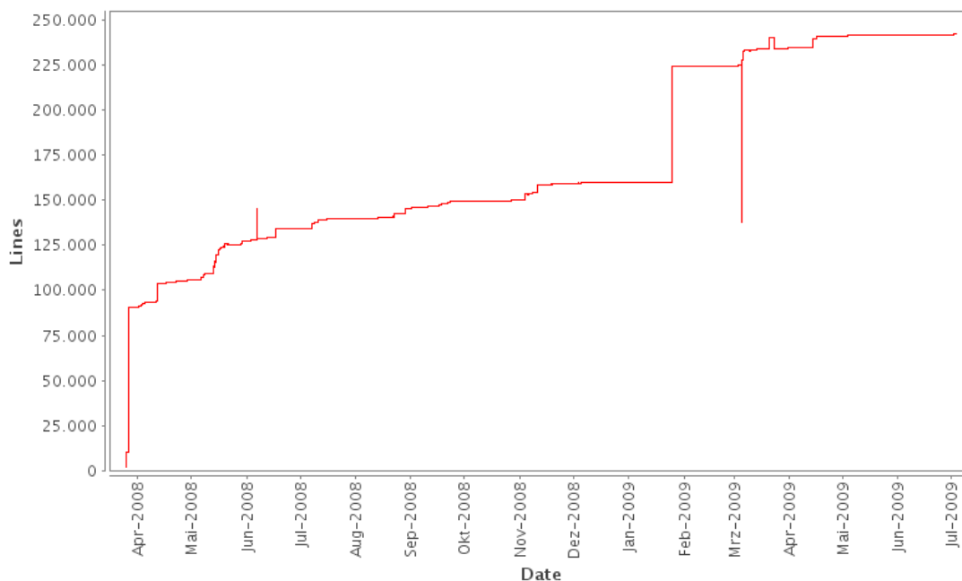
Figure 1: Lines of code of the openqc-project
